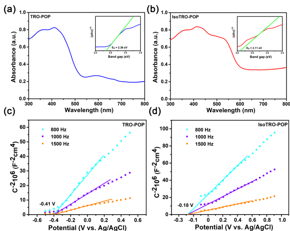
Fig. 2 (a) UV-vis diffuse reflectance spectra (DRS) and Tauc plot calculating the optical band gap (inset) of TRO-POP. (b) UV-vis diffuse reflectance spectra (DRS) and Tauc plot calculating the optical band gap (inset) of IsoTRO-POP. (c) Mott-Schottky plots of TRO-POP at frequencies 0.8, 1.0, and 1.5 kHz in a 0.2 M Na 2 SO 4 solution (pH = 7). (d) Mott-Schottky plots of IsoTRO-POP at frequencies 0.8, 1.0, and 1.5 kHz in a 0.2 M Na 2 SO 4 solution (pH = 7).
