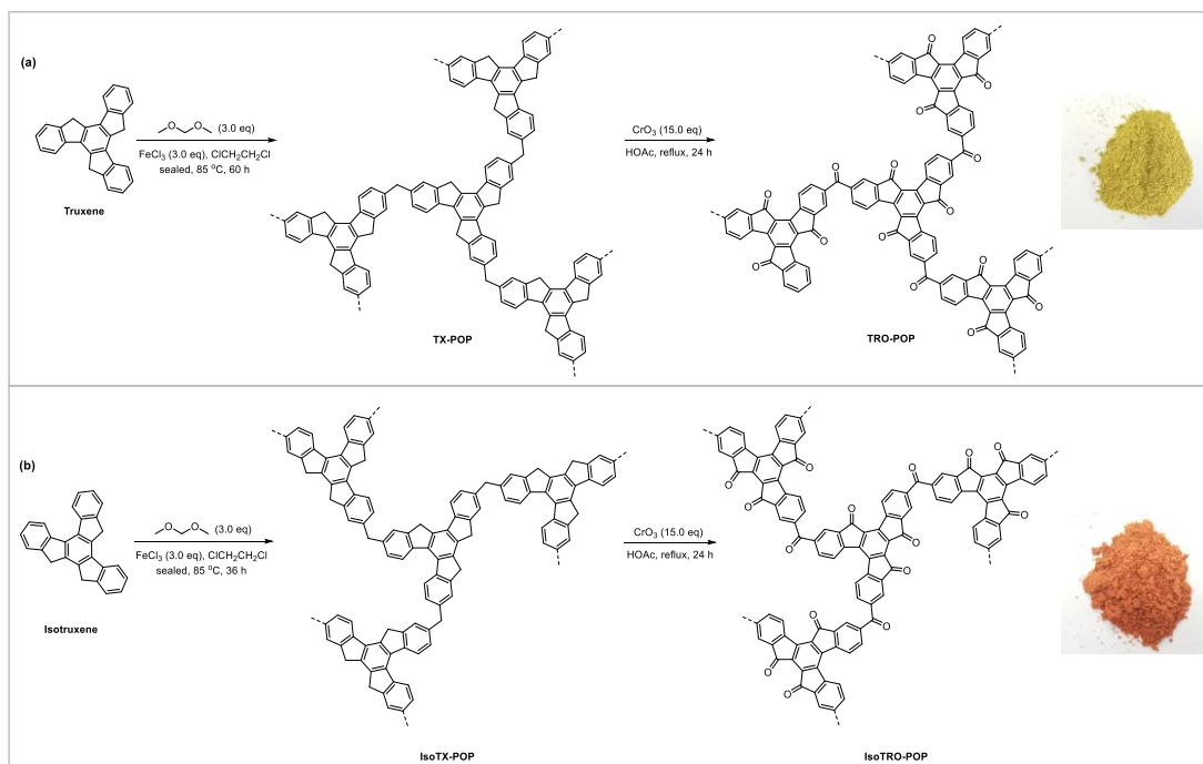
Scheme 1 Synthetic routes and idealized structures of TRO-POP and IsoTRO-POP.
