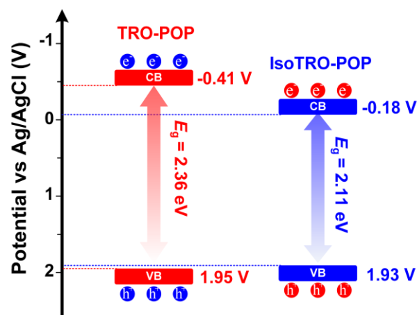
Fig. 3 Band energy diagram of TRO-POP and IsoTRO-POP.
