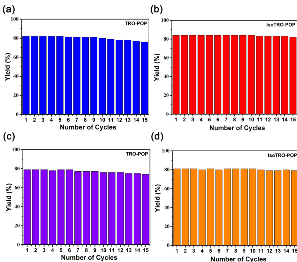
Fig. 5 (a) and (b) Recyclability tests of TRO-POP and IsoTRO-POP in the benzylic fluorination reaction. Reaction conditions: 1a (0.2 mmol), Selectfluor (0.24 mmol) in CH 3 CN (2.0 mL, 0.1 M) were stirred at room temperature under the irradiation with a 12 W CFL. (c) and (d) Recyclability tests of TRO-POP and IsoTRO-POP in the benzylic oxidation reaction. Reaction conditions: 1a (0.2 mmol), Selectfluor (0.24 mmol) in CH 3 CN/H 2 O (1:1, 0.1 M) were stirred at room temperature under the irradiation with a 12 W CFL.
