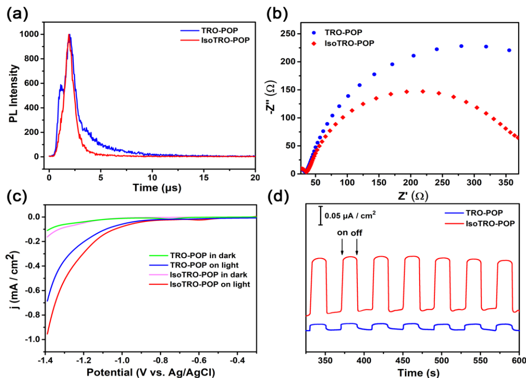
Fig. 4 (a) Time-resolved PL spectra for TRO-POP and IsoTRO-POP. (b) EIS Nyquist plots of TRO-POP and IsoTRO-POP. (c) LSV curves of TRO-POP and IsoTRO-POP under visible-light irradiation and in the dark. (d) Photocurrent tests.
