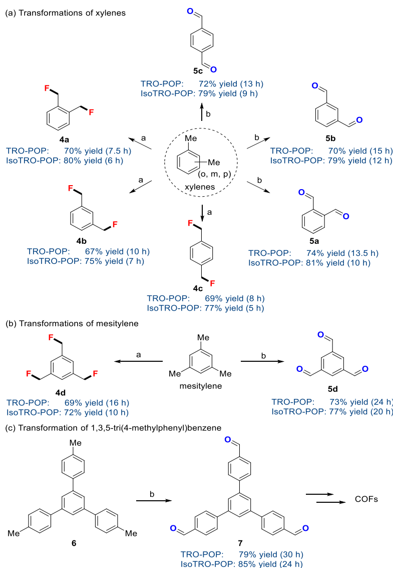
Figure 5 Transformations. Condition a: 1 (0.2 mmol), Selectfluor (0.48 or 0.72 mmol) in CH 3 CN (0.1 M) were stirred at room temperature under the irradiation with a 12 W CFL. Condition b: 1 (0.2 mmol), Selectfluor (0.48 or 0.72 mmol) in CH 3 CN/H 2 O (1:1, 0.1 M) were stirred at room temperature under the irradiation with a 12 W CFL.
